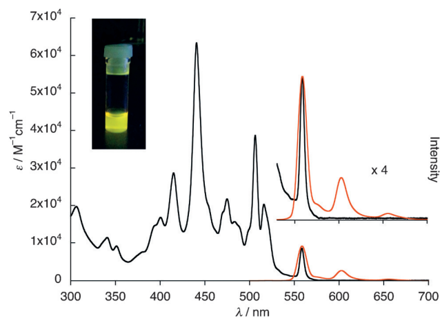
Figure 2. UV/Vis absorption (black line) and fluorescence (red line) spectra of 1 in toluene at 25^\circ\text{C} . Inset shows a photograph of toluene solution of 1 irradiated at \lambda = 365 \text{ nm} .
